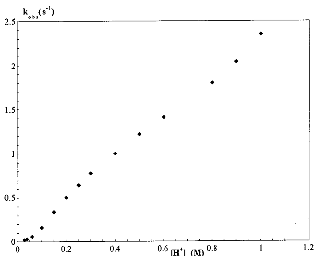
Figure 9. k_{\text{obs}} ( \text{s}^{-1} ) as a function of [\text{H}^+] (M) in the acid hydrolysis kinetics of the \text{Fe}^{\text{III}}\text{L}_3 complex, [\text{FeL3}] = 0.5 mM; solvent: water; I = 2.0 M ( \text{HClO}_4 + \text{NaClO}_4 ), T = 25^\circ\text{C}
