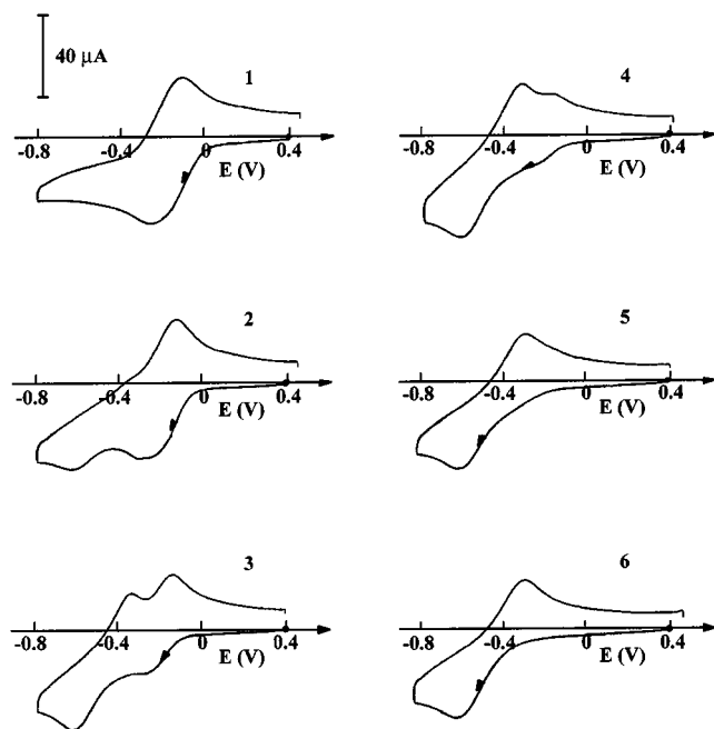
Figure 6. CV curves of Fe^{III} + L3 (2.9 mM) in H_2O + NaClO_4 0.1 M at a GC electrode (5 mm diameter); scan rate 0.1 V s -1 ; E vs. Ag/AgCl, aqueous NaCl (3 M) (+ 0.21 V vs. NHE); pH = 4.2 (1), 5.4 (2), 6.3 (3), 7.0 (4), 8.3 (5), 9.2 (6) (adjusted with HClO_4 or NaOH)
