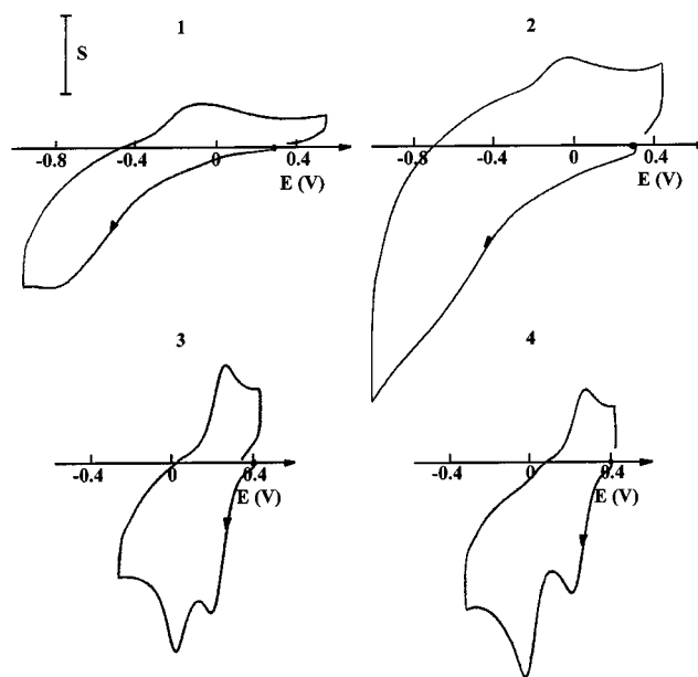
Figure 7. CV curves of Fe^{III} + L2 (1, 3) and Fe^{III} + L1 (2, 4), 0.5 mM in H_2O + NaClO_4 0.1 M at a GC electrode (5 mm diameter); scan rate 0.1 V s -1 ; E vs. Ag/AgCl, aqueous NaCl (3 M) (+ 0.222 V vs. NHE); pH = 8.3 (1, 2), 3.0 (3, 4) (adjusted with HClO_4 or NaOH); scale (S) = 10 \mu A (1, 2), 4 \mu A (3, 4)
