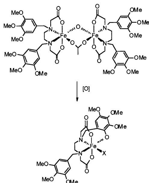
Figure 2. Reaction scheme for the oxidation of \text{Fe}_2(\text{L1})_2
