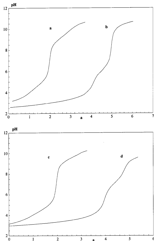
Figure 3. Potentiometric titration curves for (a) 1 mM ligand L3 ; (b) L3 + \text{Fe}^{3+} 1:1, 1 mM; (c) 1 mM ligand L1 ; (d) L1 + \text{Fe}^{3+} 1:1, 1 mM; a = mol of base added per mol of ligand; all solutions were at 25 °C and I = 0.1 M ( \text{NaClO}_4 ); the data were refined by the SUPERQUAD program ( \sigma_{\text{fit}} = 3.5\text{--}4.5 )
