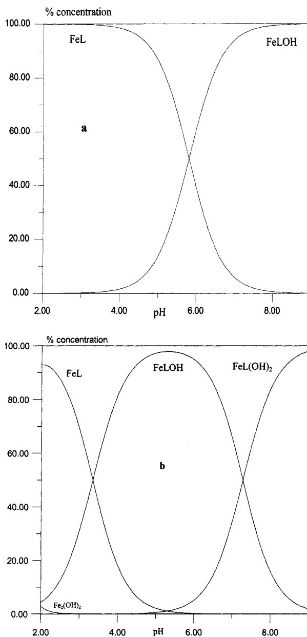
Figure 5. Distribution diagrams of the system \text{Fe}^{\text{III}} - L3 (a) and \text{Fe}^{\text{III}} - L1 (b) as a function of pH; [\text{Fe}^{3+}] = 1 \text{ mM} , [\text{ligand}] = 10 \text{ mM}
