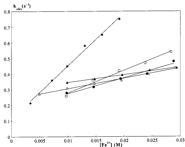
Figure 8. Variation of the experimental rate constant k_{\text{obs}} ( \text{s}^{-1} ) for the formation of the \text{Fe}^{\text{III}}\text{L}_3 complex as a function of [\text{Fe}^{3+}] (M) at various [\text{H}^+] (M): (◆) 0.05 , (□) 0.08 , (●) 0.10 , (Δ) 0.125 , (▲) 0.15 ; [\text{L3}] = 0.4 mM; solvent: water, I = 2.0 M ( \text{HClO}_4 + \text{NaClO}_4 ), T = 25^\circ\text{C}
