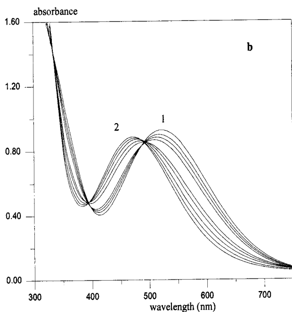
Figure 4. UV/Vis absorption spectra of \text{Fe}^{3+} - L3 as a function of pH; (a) 1: pH = 0.9; 2: pH = 1.8; (b) 1: pH = 4.5; 2: pH = 6.5; [\text{Fe}^{3+}] = [\text{L3}] = 0.5 \text{ mM} ; I = 0.1 \text{ M} ( \text{NaClO}_4 )
