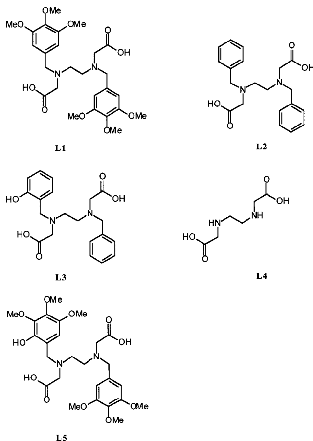
Figure 1. Structure of the ligands L_n
